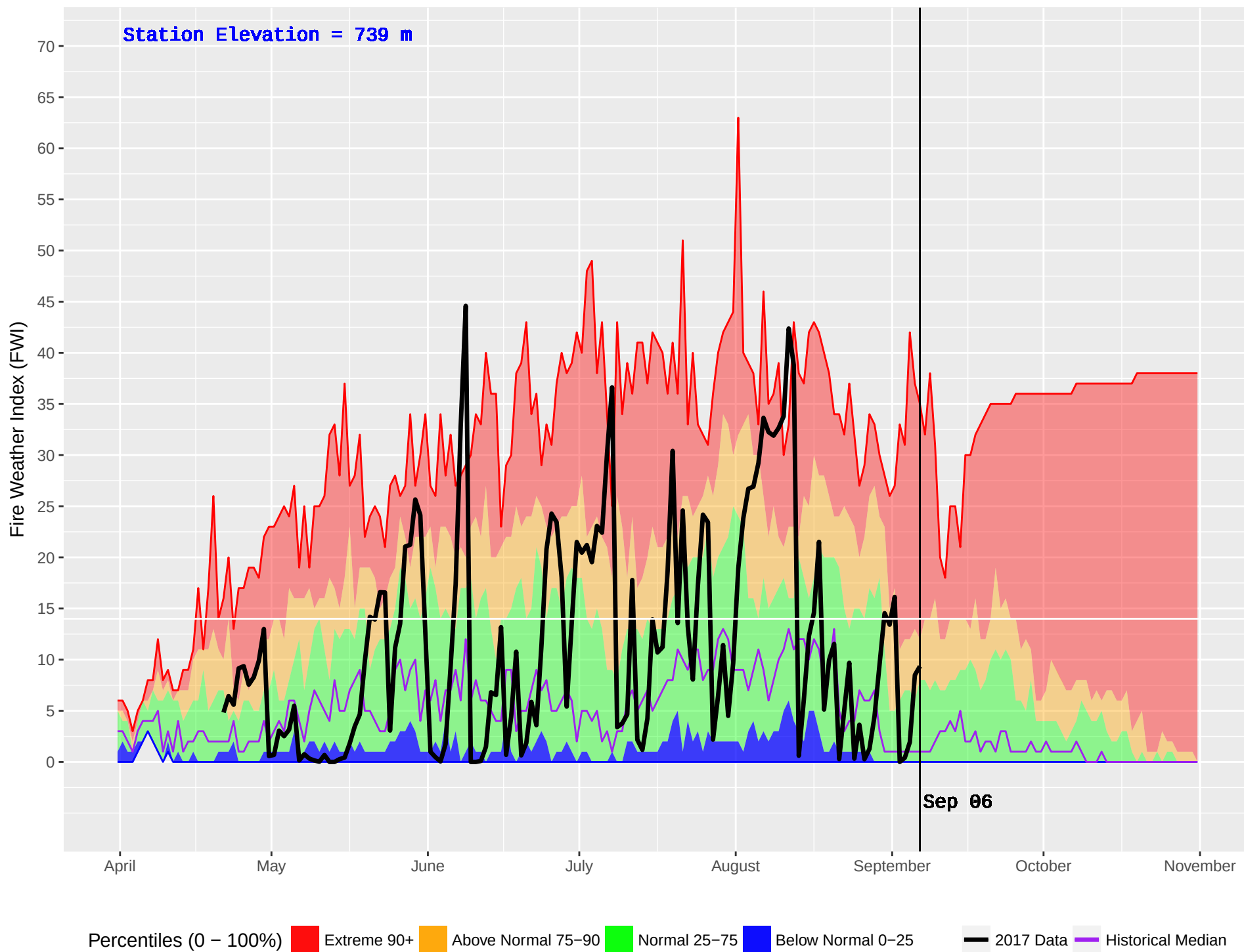
BEAR LAKE (149) : Historical (1980–2016) and Current (2017) Noon Fire Weather Index (FWI)
